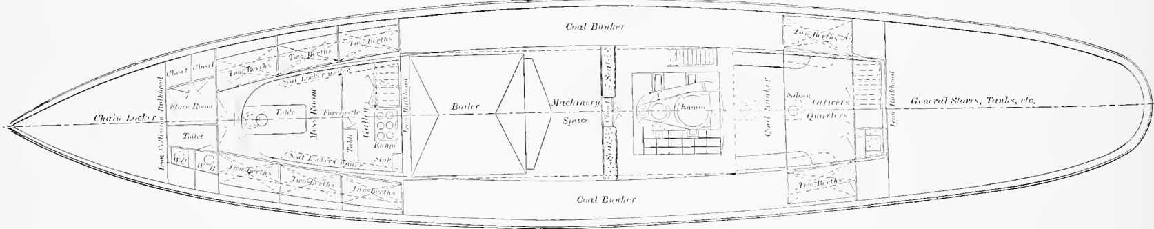
PLANS FOR AN IRON TUG.—Designed by Henry J. Gielow, New York.
